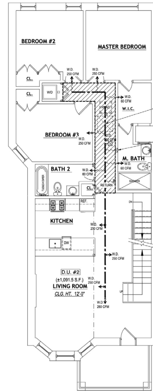
2ND FLOOR SCALE
