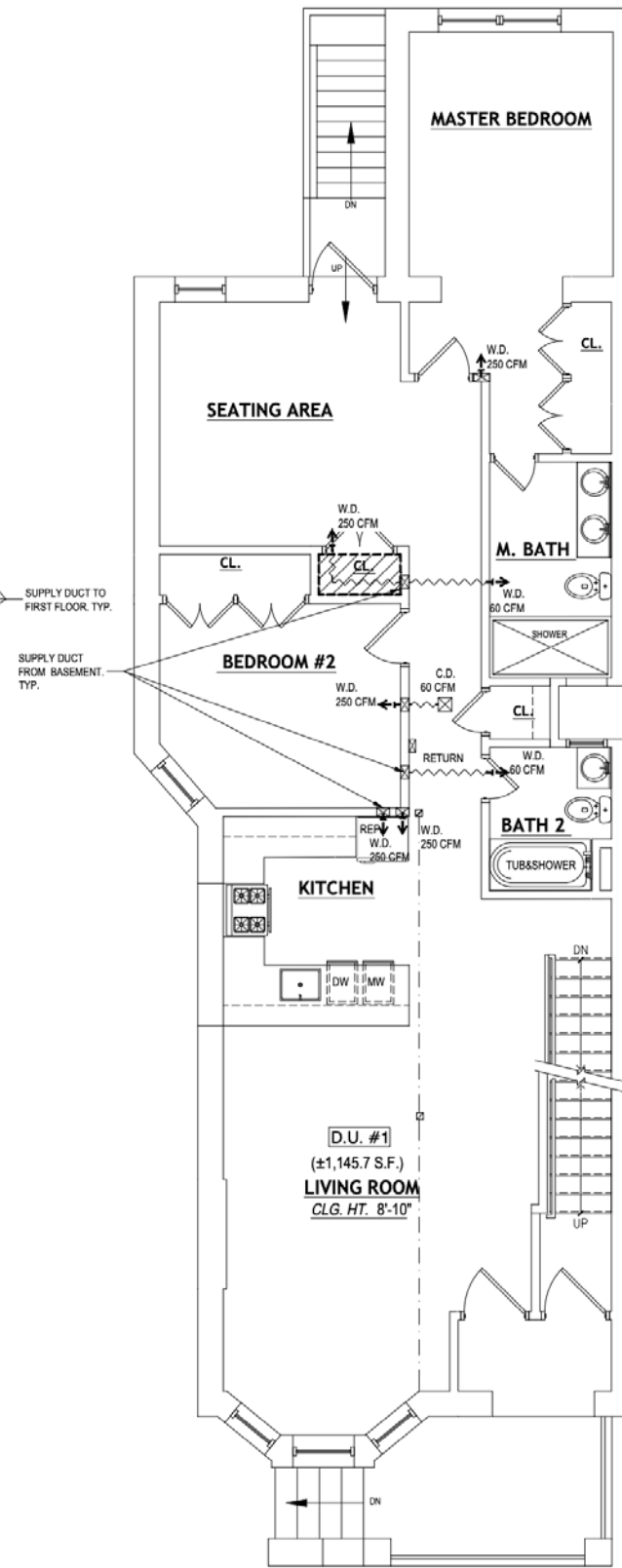
1ST FLOOR SCALE
